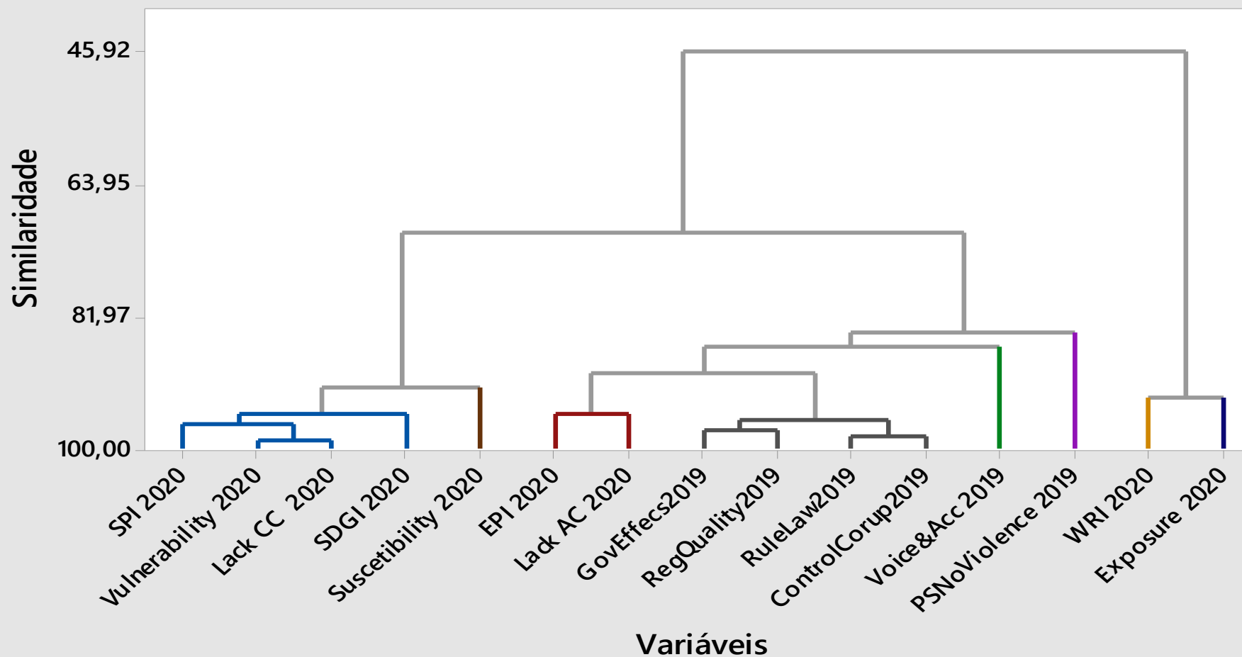
Dendrogram showing clusters of variables based on correlations
